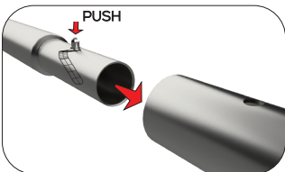
Press button & insert swaged end into receiving end of tubing
