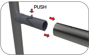
Attach the female tube in the right position and push the button, and slide the tube
