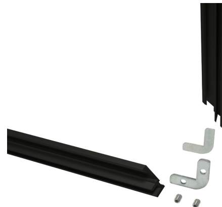
Corner Connection
