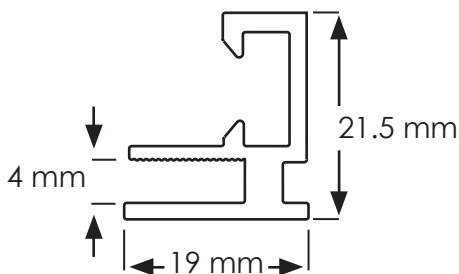
*Split Connector
